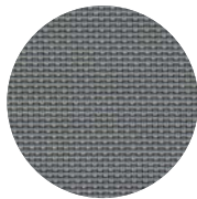
Shale
